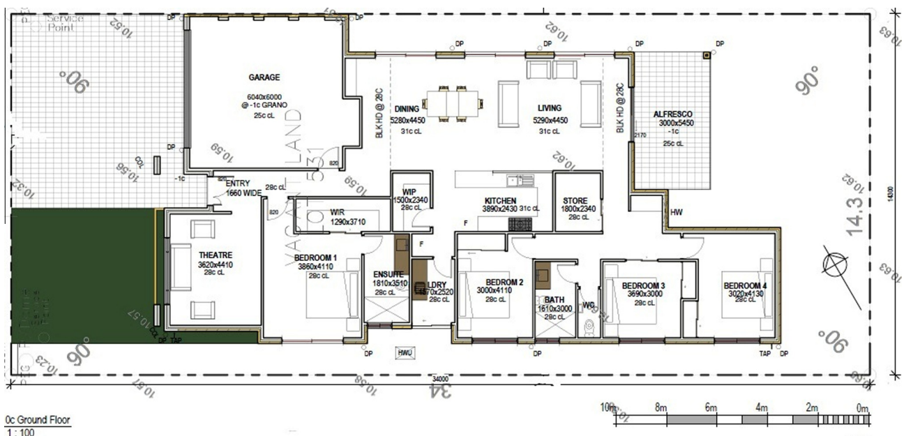
Figure 1. Floor plan of a typical 4 \times 2 \times 2 house in Perth.
